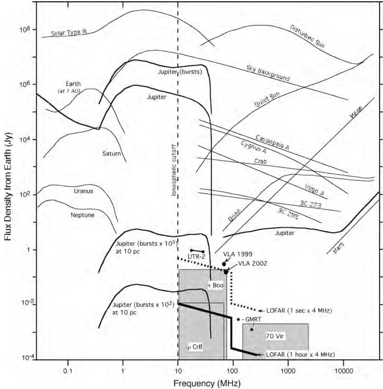
Figure 17 : Spectra of astronomical radiosources detected from the Earth's vicinity ( 1 \text{ Jansky} = 1 \text{ Jy} = 10^{-26} \text{ Wm}^{-2}\text{Hz}^{-1} ). Planetary spectra, corresponding to auroral radio emissions, are deduced from Voyager and Cassini measurements. Jupiter's average flux density is about 10^6 \text{ Jy} , while peak flux densities reach or exceed 10^7 \text{ Jy} during short-lived bursts. If all planetary emissions were normalized to the same observer distance of 1 AU, Jupiter's spectrum should be upscaled by \times 20 , Saturn's by \times 100 , Uranus' by \times 400 , and Neptune's by \times 900 , so that all are grouped within 2-3 orders of magnitude of each other. Jupiter's peak spectrum is reproduced with two different scalings to illustrate the possible radio spectrum of hot Jupiters. Shaded boxes are published predictions from a few candidate exoplanets. Sensitivities of UTR-2, VLA, GMRT and future LOFAR observations are indicated. The Earth's ionospheric cutoff is indicated at 10 MHz.
