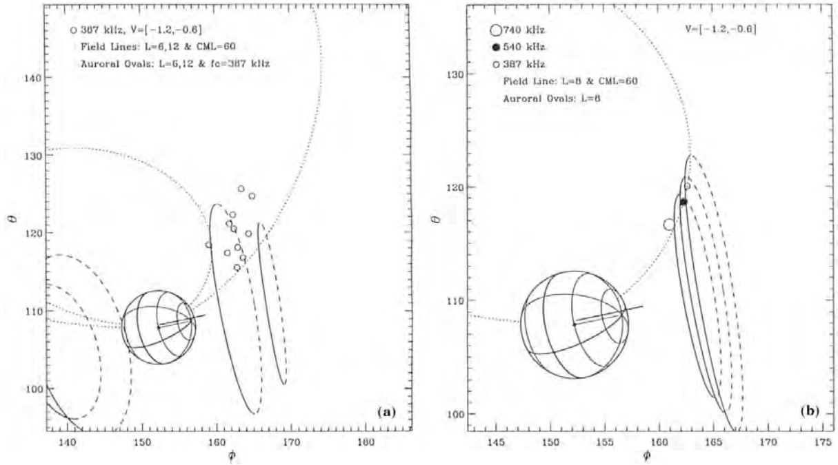
Figure 12 : Goniometric results from Ulysses near Jupiter on 1994/02/08, from 12 RJ ( \sim 106 km) from the planet. (a) The direction of the dominant hectometre RH circular source at 387 kHz measured during 12-sec intervals over a 35 minute-period is plotted as open dots in the frame of Ulysses radio antennas. Jupiter is represented with its rotation axis (lightface) and its magnetic axis (boldface) pointing to the North. Dotted lines are dipole magnetic field lines with apex at 6 and 12 RJ. Auroral ovals crossing these field lines at a local electron cyclotron frequency f_{ce} = 387 kHz are solid/dashed lines (visible/hidden portion from Ulysses). (b) Average source directions over the same 35-min interval at 387, 540, and 740 kHz. The dotted dipolar field line with apex at 6 RJ crosses the 3 radio sources at the same point as the corresponding northern auroral ovals along which f_{ce} = 387 , 540, and 740 kHz with increasing distance from the planet (solid/dashed). This measurement by Ladreiter et al. [1994] is the first direct proof that hectometre emission is produced at/near the local f_{ce} on the X mode (RH polarization from northern magnetic hemisphere). The geometry allows to deduce the 3D source location and radio beaming angle.
