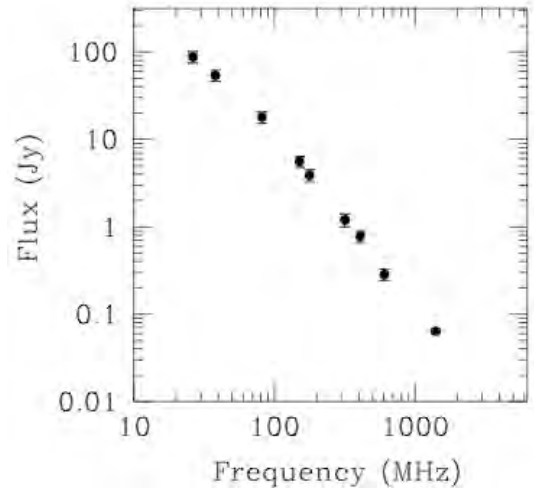
Figure 3 : Integrated spectrum of the diffuse radio source in A1914 (Bacchi et al, 2003; Komissarov & Gubanov 1994)
