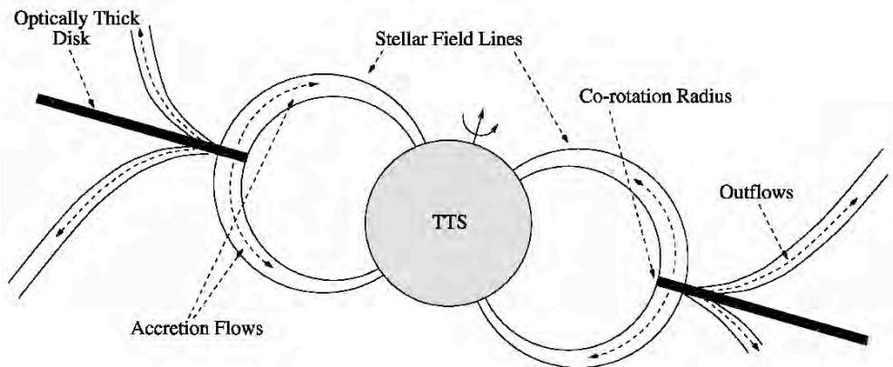
Fig. 2. Schematic illustration of the “magnetospheric accretion” process, widely thought to take place in T Tauri stars, and probably also in protostars (Stassun 2001).
