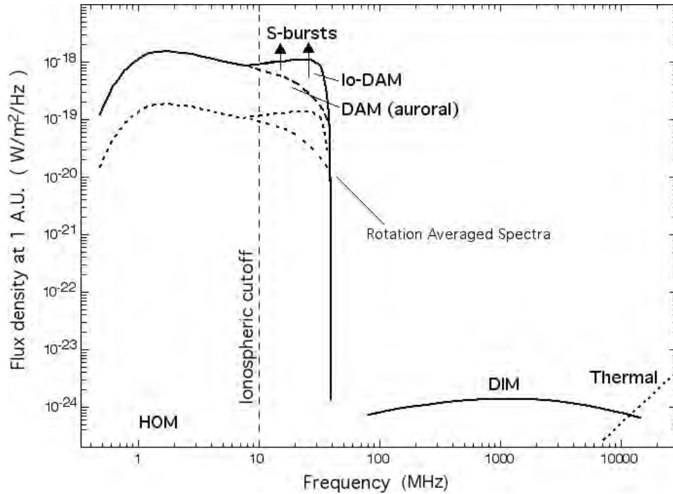
Figure 11: Spectra of Jovian radio components observable from the Earth's vicinity. « DIM' » represents the decimeter synchrotron emission from the radiation belts. DAM emission consists of the superposition of auroral-DAM (dashed), which extends down to the hecto-kilometer range, and Io-DAM (solid). Part of Io-DAM consists of impulsive bursts (S-bursts). The Earth's ionospheric cut-off lies on the average about 10 MHz. The sharp cut-off at 40 MHz corresponds to the maximum electron cyclotron frequency at the planetary surface. Dotted lines represent rotation-averaged spectra at times of intense activity (or equivalently typical averages over emission intervals). Solid/dashed lines represent peak intensities detected during active periods.
