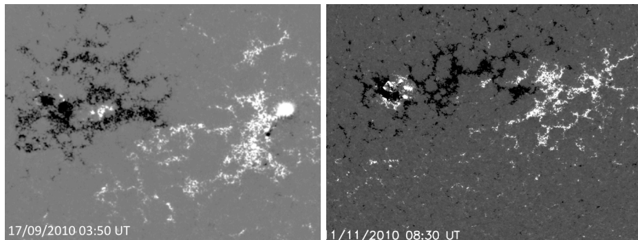
Figure 2: Emerging flux inserted in the negative following polarity of mature ARs during the rising phase of the solar cycle 24 observed with SDO/HMI magnetograph. Left panel: AR on 17 September 2010 at 03:50 UT. Right panel: AR on 11 November 2010 at 08:30 UT. White/black regions are positive/negative longitudinal magnetic field.
