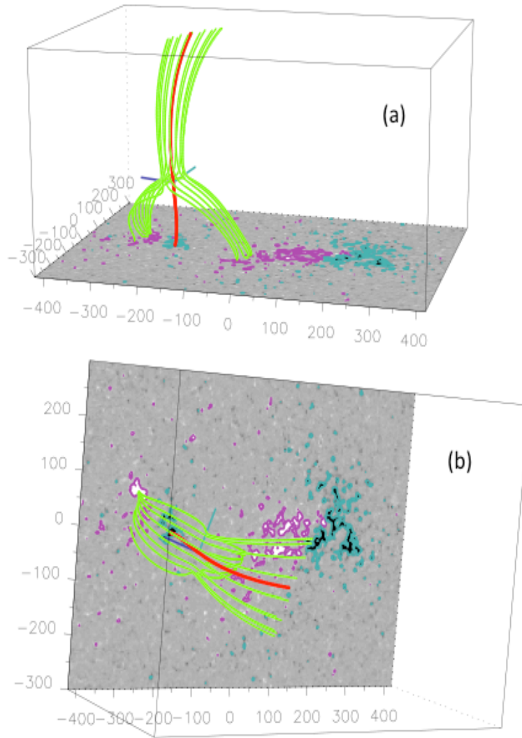
3 4 Figure 8 Location of a high-altitude (about 130 Mm) null point above AR2 in the AR1-AR2 5 complex in a Cartesian potential field extrapolation. The spine field line (red) and fan field lines 6 (green lines) are shown from two perspectives (a) from the South and (b) as seen from Earth. 7 The bottom boundary is an MDI magnetogram taken on 9 January 2008, when the AR1-AR2 8 complex was closest to the central meridian. Negative polarity is contoured with turquoise, 9 positive with magenta.
