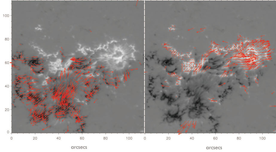
Figure 5. Photospheric flow horizontal velocities on negative (left) and positive (right) polarities. Red arrows represent velocities up to 3 \text{ km s}^{-1} with the background being the average image with positive (white) and negative (black) polarities (saturated at \pm 2500 \text{ G} ). The flow maps were derived from LCT analysis in the interval 12:00 to 13:00 UT employing a FWHM correlation window of 3'' .
