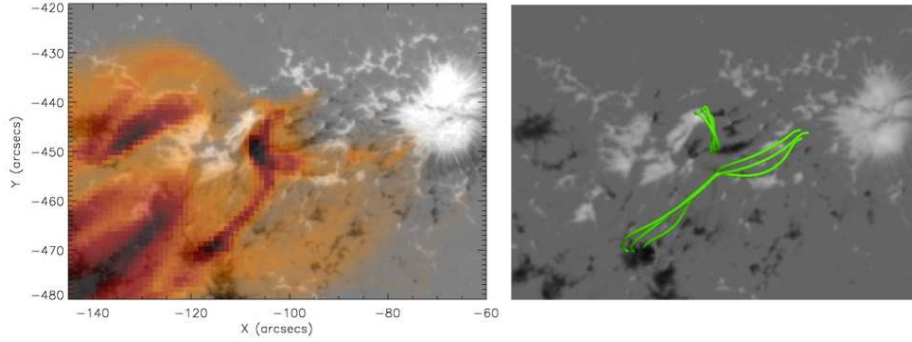
Figure 12. Left: XRT image obtained with the Ti poly filter on 4 July 2009 at 11:52 UT, aligned on the SOT/SP LOS image of 4 July 2009 at 11:58 UT, in reversed colour scale. Right: Same reconnected field lines as the green field lines in Figure 10c,d, projected on the plane of the sky.
