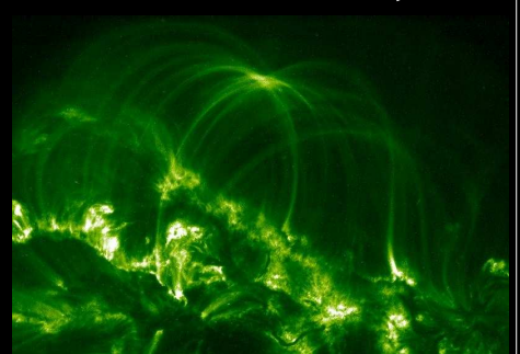
Satellite TRACE/NASA, EUV
