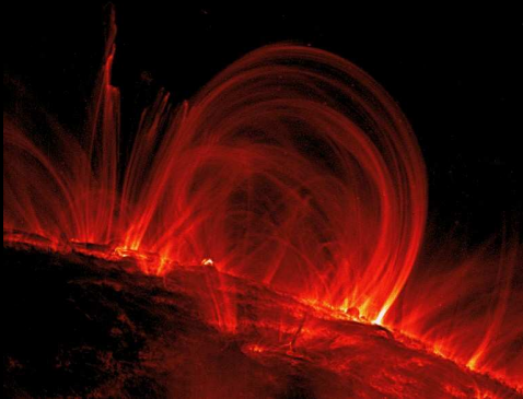
Satellite TRACE/NASA, EUV
