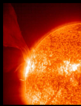
Approximate size of earth for comparison
