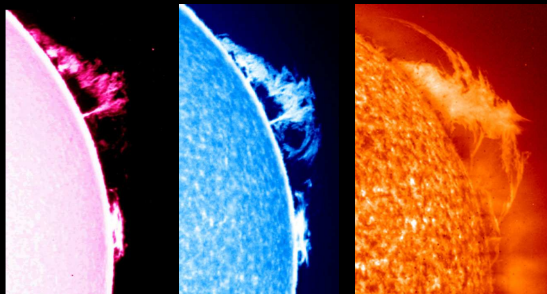
H \alpha Meudon
