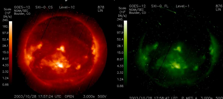
Rayons X mous, satellite GOES
