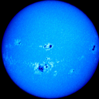
CaII K1v Meudon
