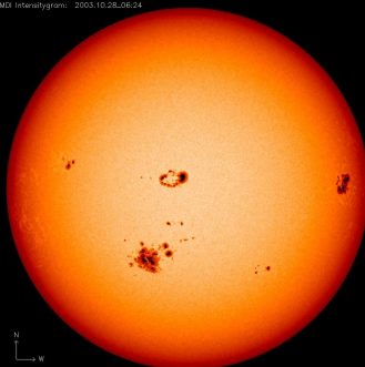
MDI Intensitygram: 2003_10_28_08:24
