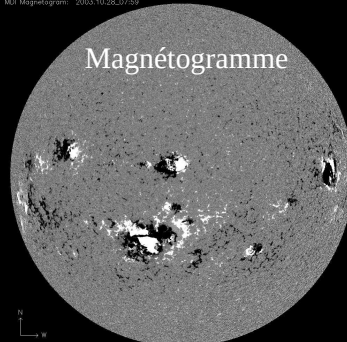
MDI Magnetogram: 2003_10_28_07:59
