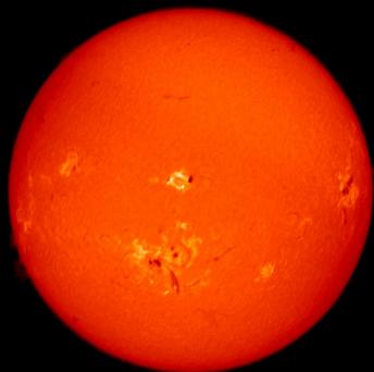
H \alpha Meudon
