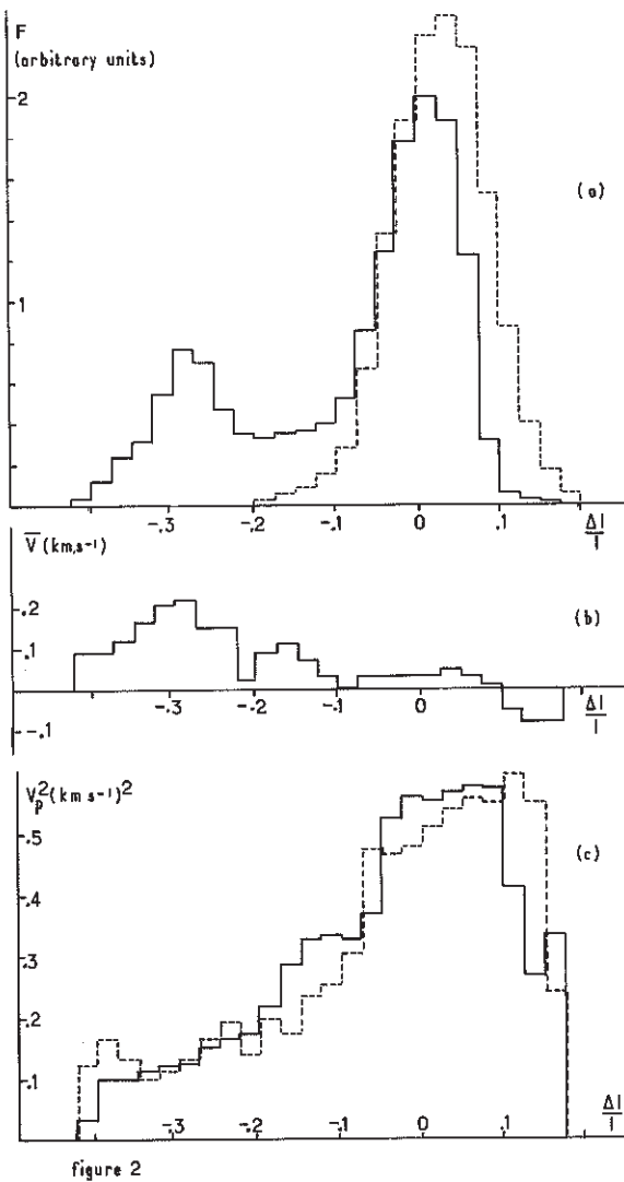
Figure 2. a Distribution function of the H \alpha intensity fluctuations at \Delta\lambda=0.3\text{\AA} (continuous line) and at \Delta\lambda=0.6\text{\AA} (dashed line). b Mean value of the steady velocities versus Intensity fluctuations (H \alpha\pm 0.3\text{\AA} ). c Variation of the mean function \bar{V}p^2 versus Intensity fluctuation for the period 300 s (continuous line) and 200 s (dashed line)
