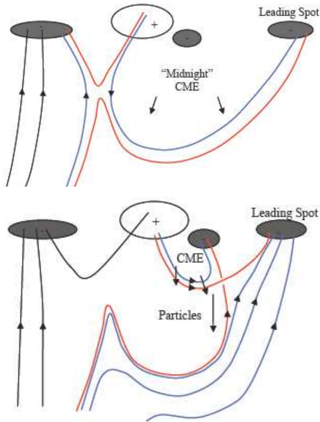
Figure 6. Cartoons showing the mechanism leading to the N burst. Top panel: formation of the dipped large-scale field lines during the “midnight” halo CME event. Note that successive loop expansions due to this CME continued for several hours (Figure 5). Bottom panel: Reconnection between magnetic loops of the two CMEs (at “midnight” and \approx 8 UT) injected accelerated electrons into the huge dipped field lines, leading to an N burst (Figure 2). Pre-reconnected field lines are in blue, and reconnected field lines are in red, while some extra field lines are added in black to outline the surrounding magnetic configuration.
