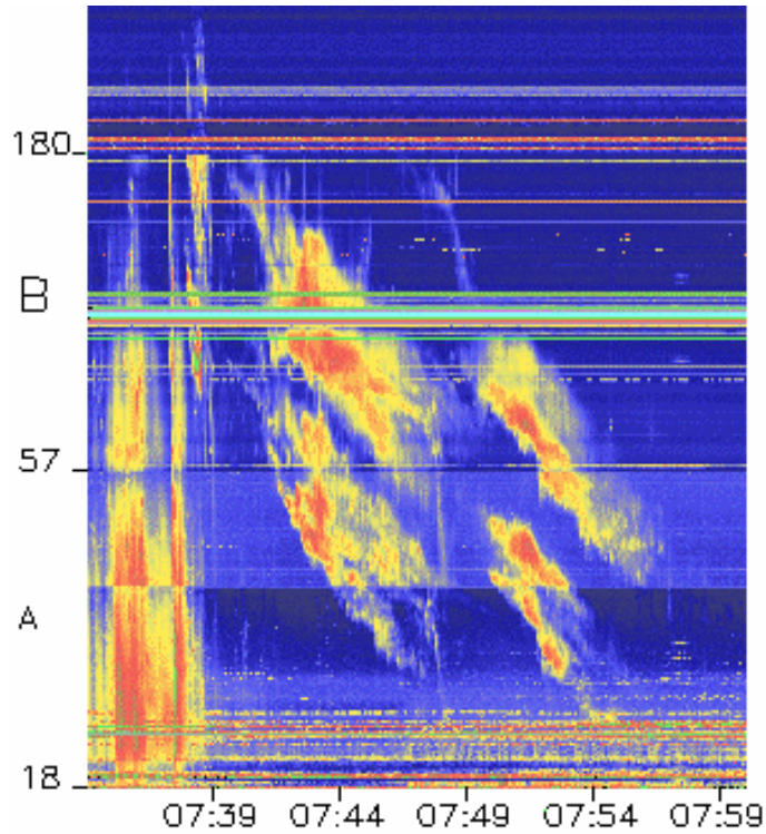
Figure 1. Culgoora dynamic radio spectrum from January 20, 2004, event (the ordinate scales as the logarithm of the frequency). The intensity increases from dark blue, green, yellow to red. A group of type III is present on the left of the image (before 7:39 UT). They are followed by two Type II bursts which drift at a similar rate. Both fundamental and first harmonic emissions are present.
