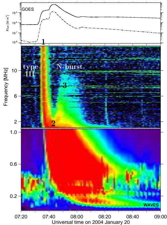
Figure 2. Type III and N-bursts observed by the WAVES instrument on the Wind spacecraft (the ordinate scales linearly with the frequency). The GOES light curve is added on the top for reference to the flare evolution. Position 1 indicates an initial Type III burst. Position 2 indicates a frequency turnover characteristic of a U-burst. Position 3 shows a further turnover. This frequency drift sequence constitutes a type N-burst. In the low frequency range, \approx 0.2 - 0.6 MHz, the noisy signal that dominates before 07:40 and after 08:30 UT is auroral emission; on the right, it covers partly the signal of the type N burst.
