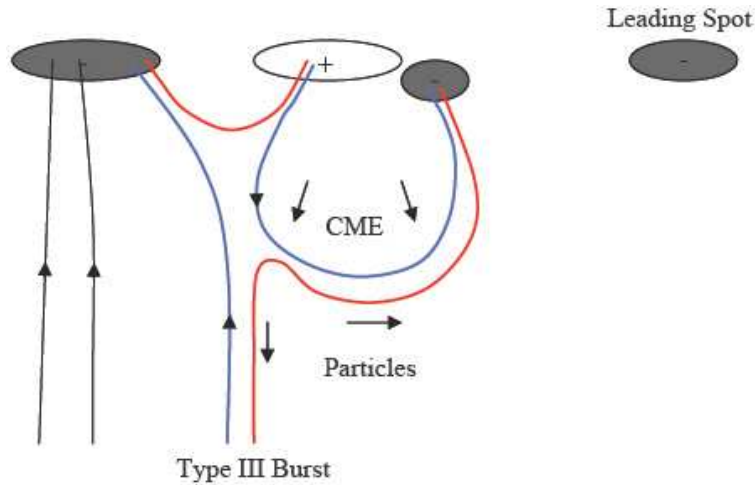
Figure 3. Schematic view of the main magnetic polarities and field line connections involved in the large-scale reconnection. The expanding magnetic structure (CME) reaches the oppositely directed magnetic structure of the streamer east of the flaring AR (blue lines). The resulting reconnection process leads to loop formation interconnecting the two neighbouring magnetic polarities and the formation of large-scale "open" field lines (red lines), along which particles accelerated during the reconnection process, propagate. The upward traveling electrons from this site produce type III bursts, while the downward traveling electrons emit reverse-slope bursts.
