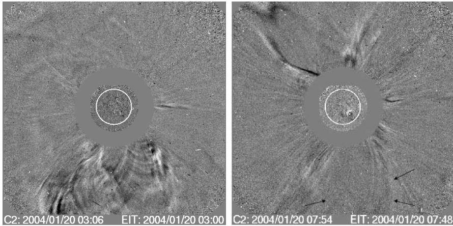
Figure 5. The “midnight” halo CME lasted for several hours in C2 field of view. A large number of loops kept expanding from the Sun, showing continuous signs of interaction with the eastward streamer (see Appendix). The last expanding loop detectable is extending to about 6 R_{\odot} in the right panel (black arrows). It is present at the time when the radio N-burst is observed.
