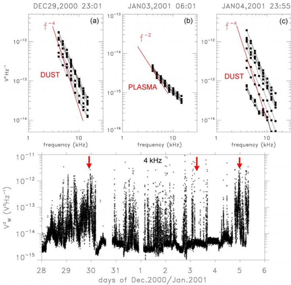
Figure 2. Power spectral density as a function of time recorded on the W antenna at 4 kHz (bottom), with corresponding power spectra (computed from \sim 0.15 s snapshots) acquired during three 3 min. intervals centered at the times indicated (top).
