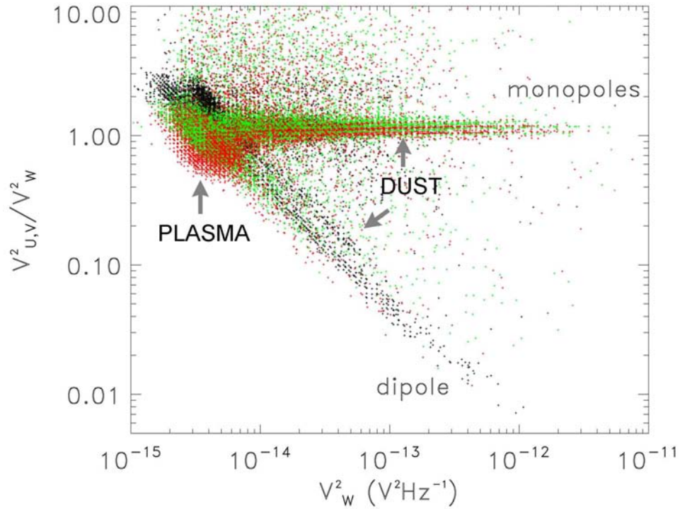
Figure 4. Ratios of the power at 4 kHz on the monopoles U and V (red and green respectively) to that on W, as a function of the latter during the period shown in Fig.2. The ratio of the power on the dipole U-V to that on the monopole W is plotted in black. The dust, which shows up above about a few 10^{-14} \text{ V}^2\text{Hz}^{-1} is seen on the monopoles with similar levels on each, whereas the dipole records only the (smaller) plasma noise. The remaining points are jovian electromagnetic emissions, whose relative intensities depend on other factors.
