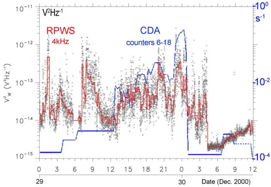
Figure 3. Power spectral density as a function of time at 4 kHz (dots), with 10 min. averages in red, proportional to the dust impact rate, compared to the rate measured with the cosmic dust analyser (blue line, adapted from [Graps et al. , 2001]).
