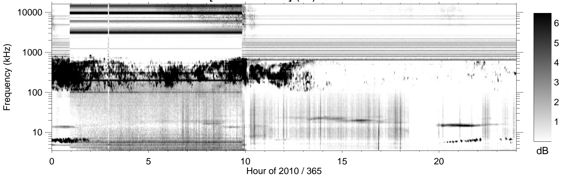
RPWS [ABCH1H2/Ex] (-B) 2010/12/31
