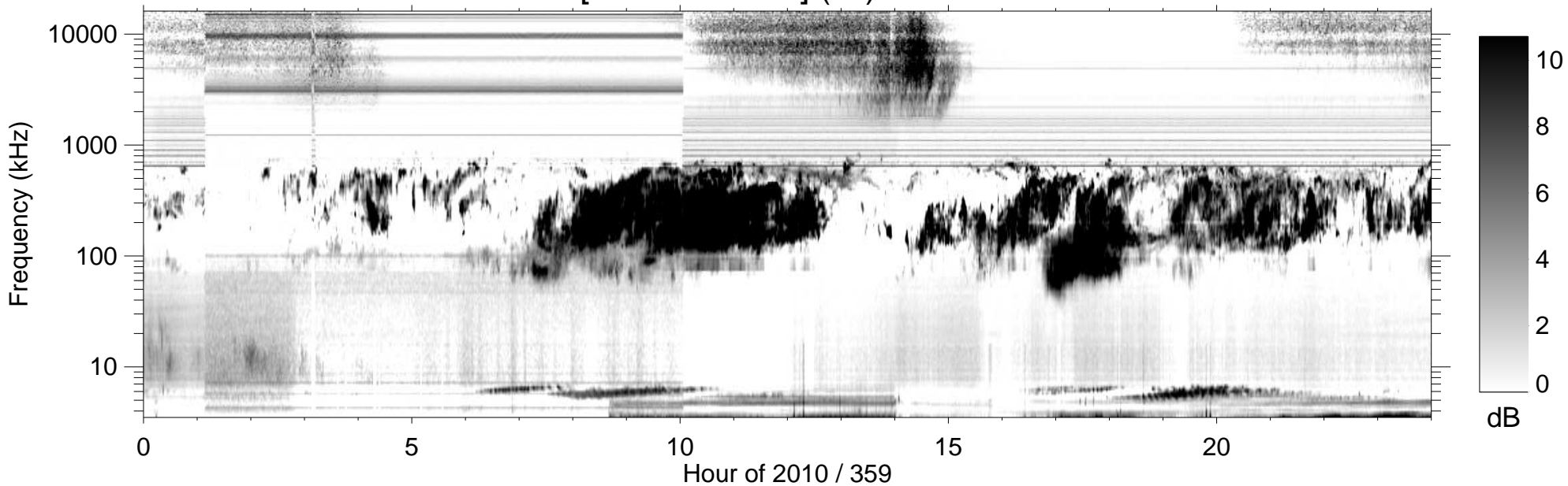
RPWS [ABCH1H2/Ex] (-B) 2010/12/25
