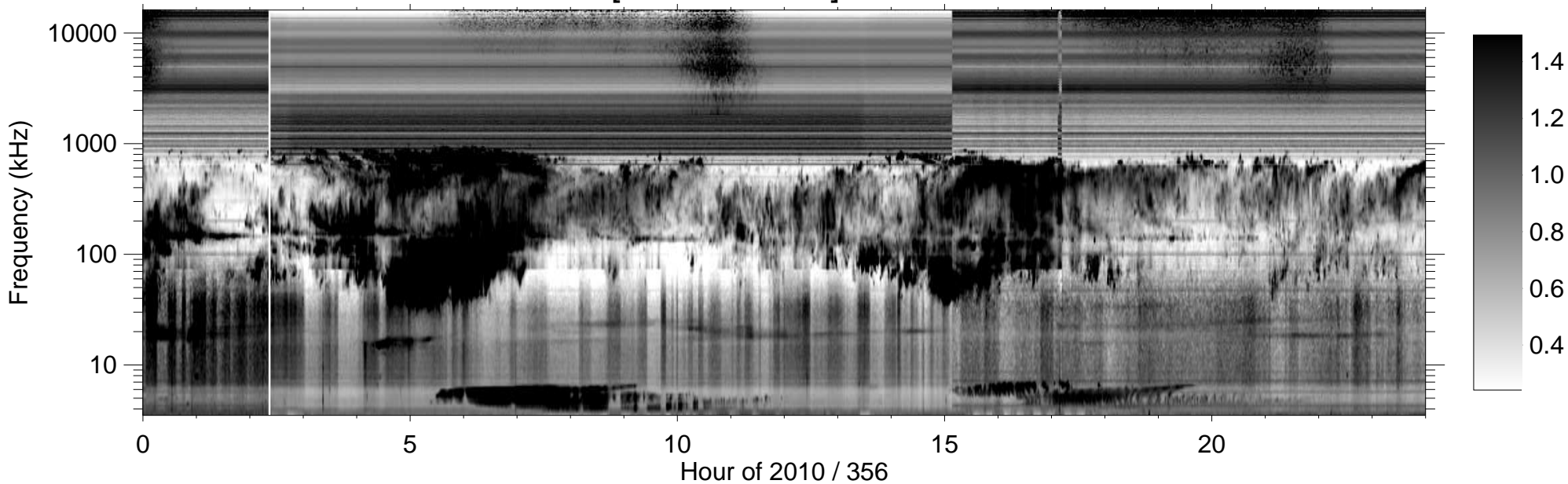
RPWS [ABCH1H2/Ex] (-B) 2010/12/22
