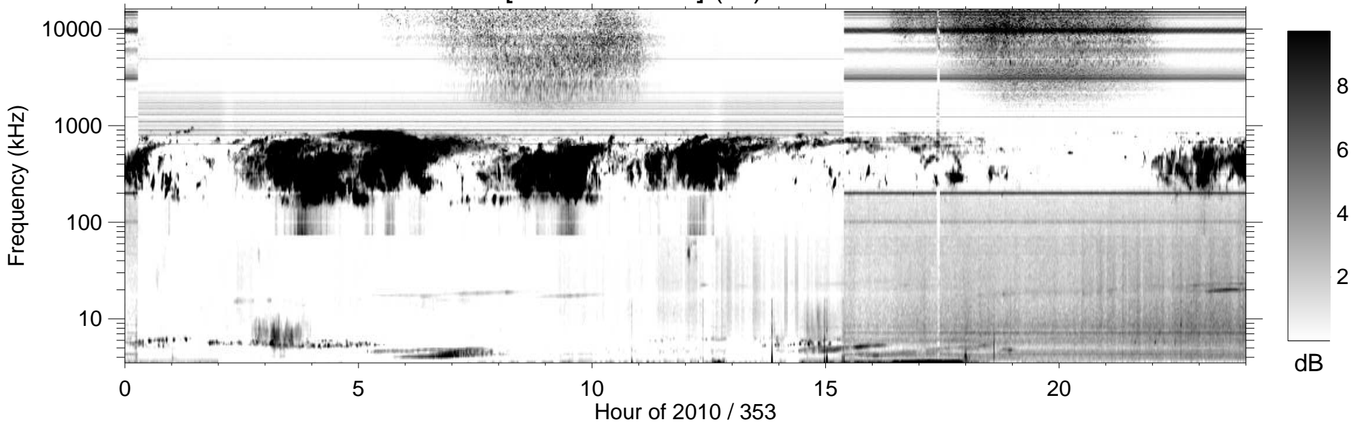
RPWS [ABCH1H2/Ex] (-B) 2010/12/19
