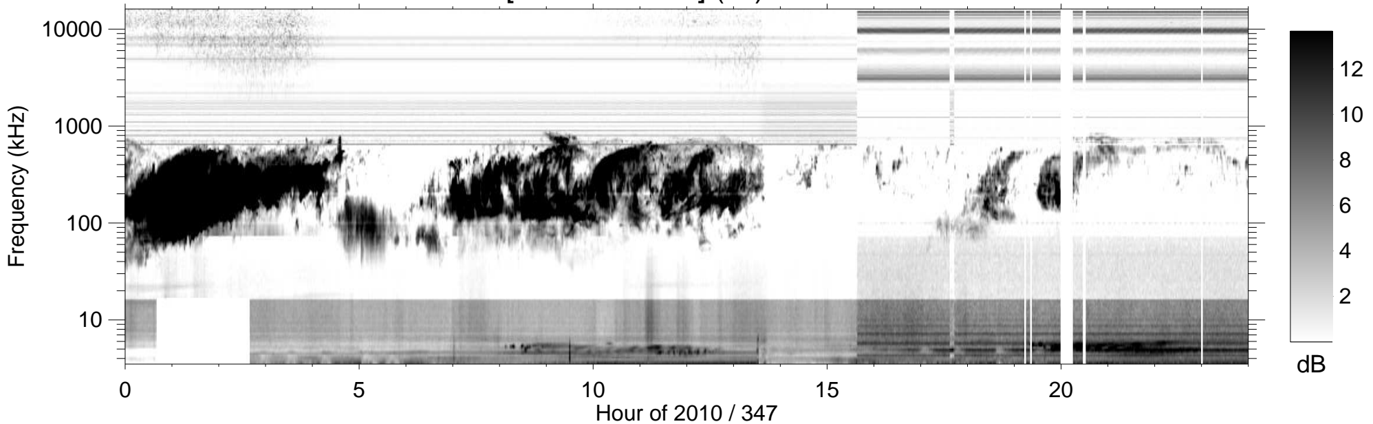
RPWS [ABCH1H2/Ex] (-B) 2010/12/13
