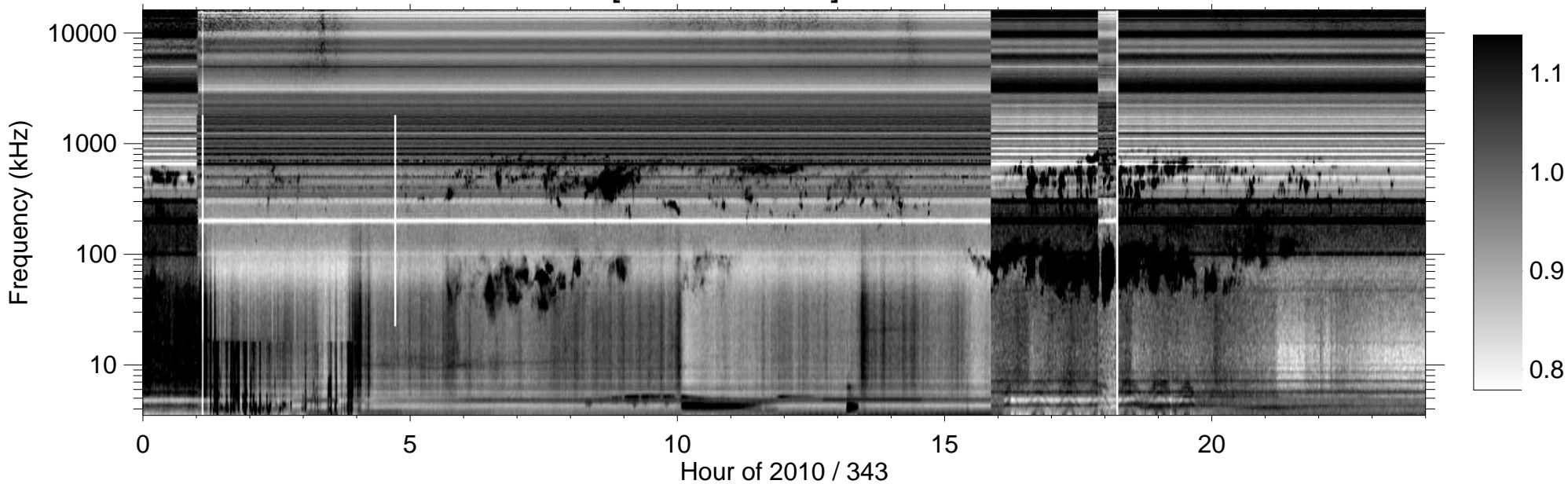
RPWS [ABCH1H2/Ex] (-B) 2010/12/09
