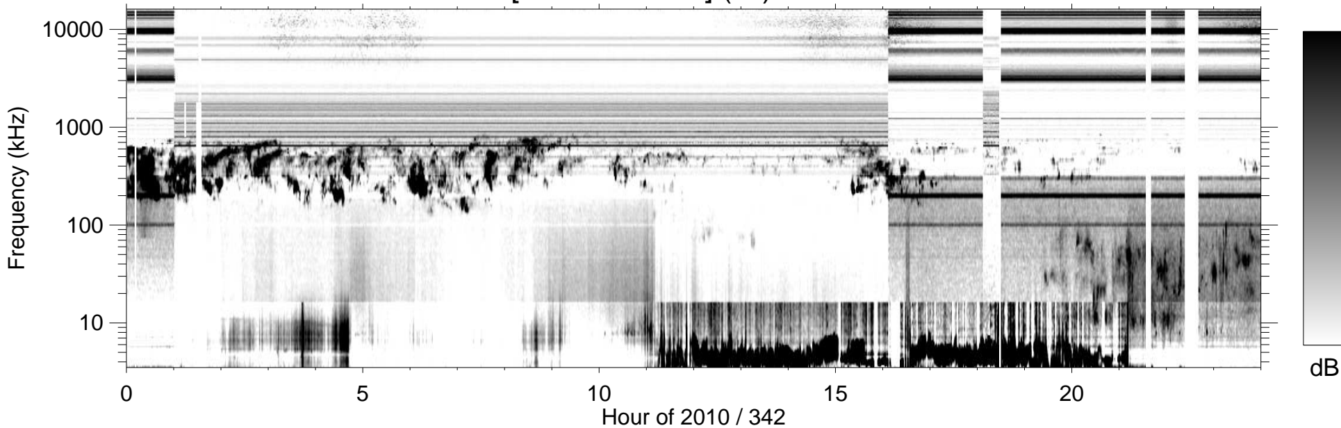
RPWS [ABCH1H2/Ex] (-B) 2010/12/08
