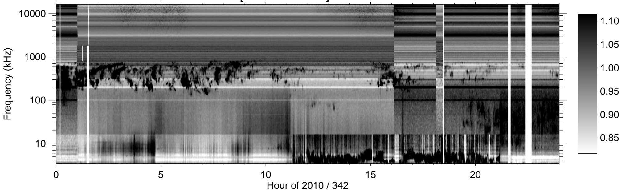
RPWS [ABCH1H2/Ex] (-B) 2010/12/08
