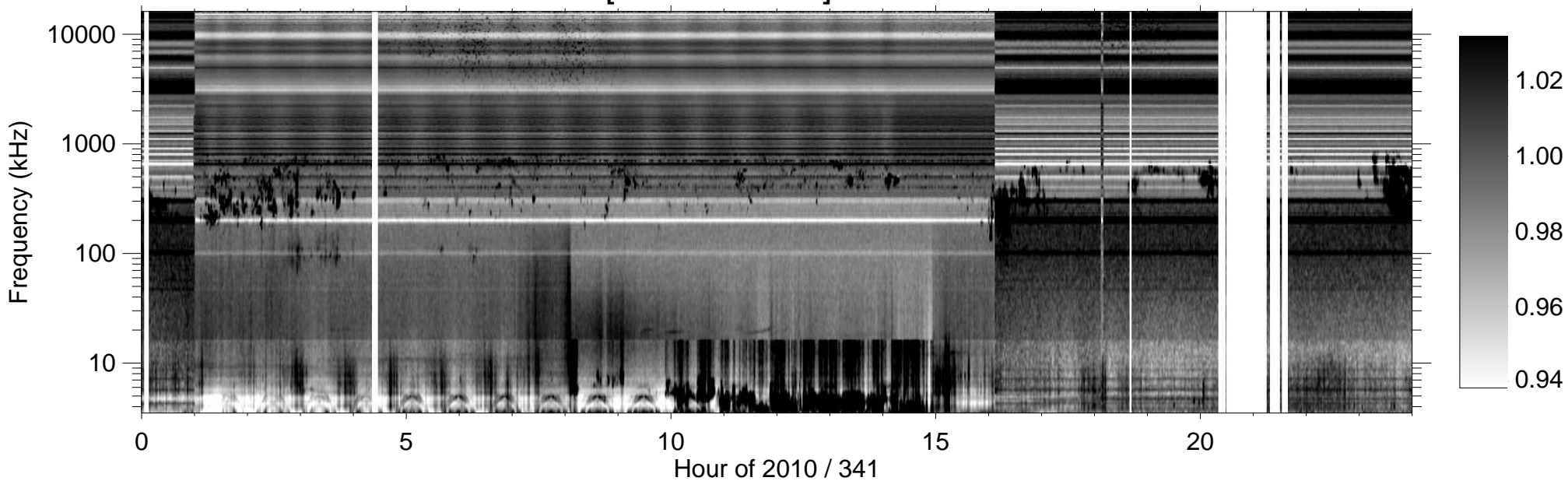
RPWS [ABCH1H2/Ex] (-B) 2010/12/07
