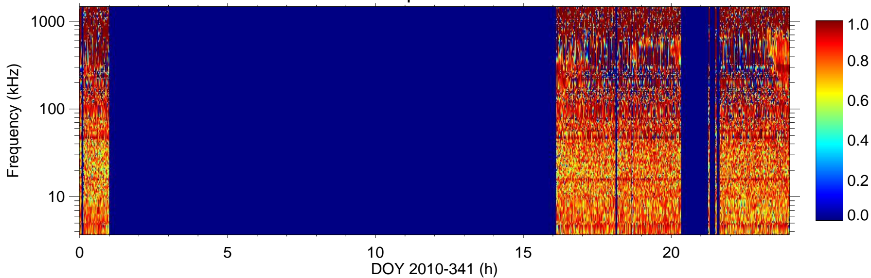
Total polarization
