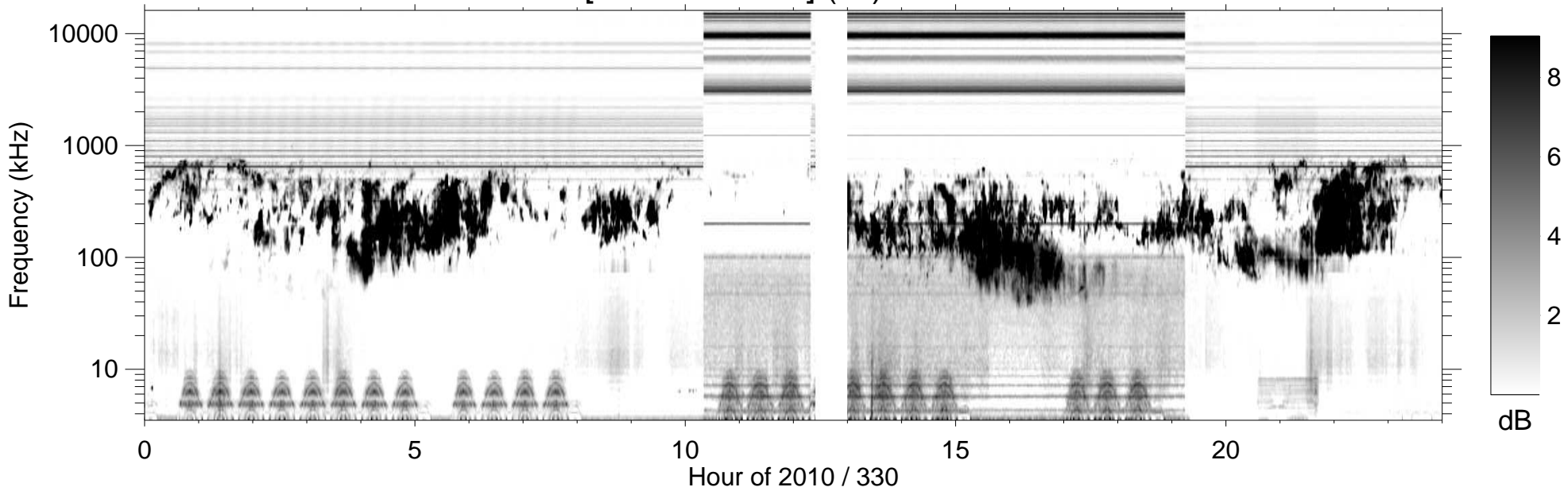
RPWS [ABCH1H2/Ex] (-B) 2010/11/26
