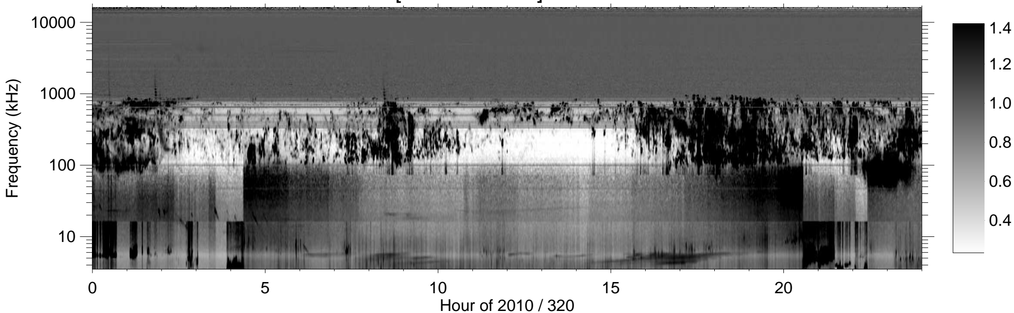
RPWS [ABCH1H2/Ex] (-B) 2010/11/16
