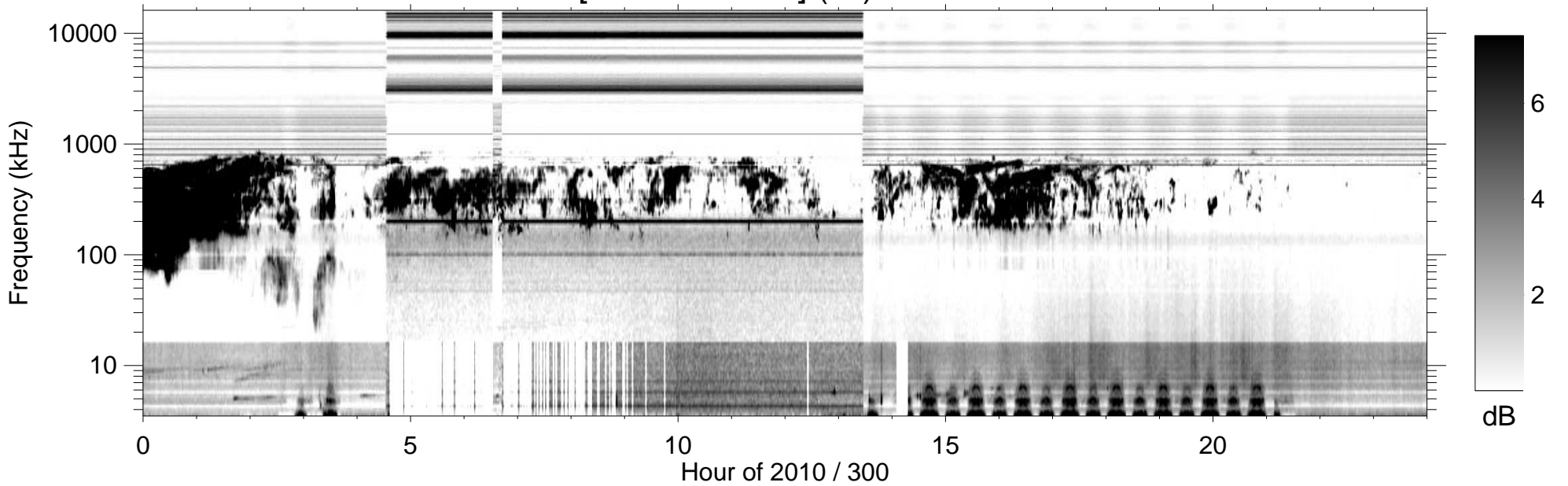
RPWS [ABCH1H2/Ex] (-B) 2010/10/27
