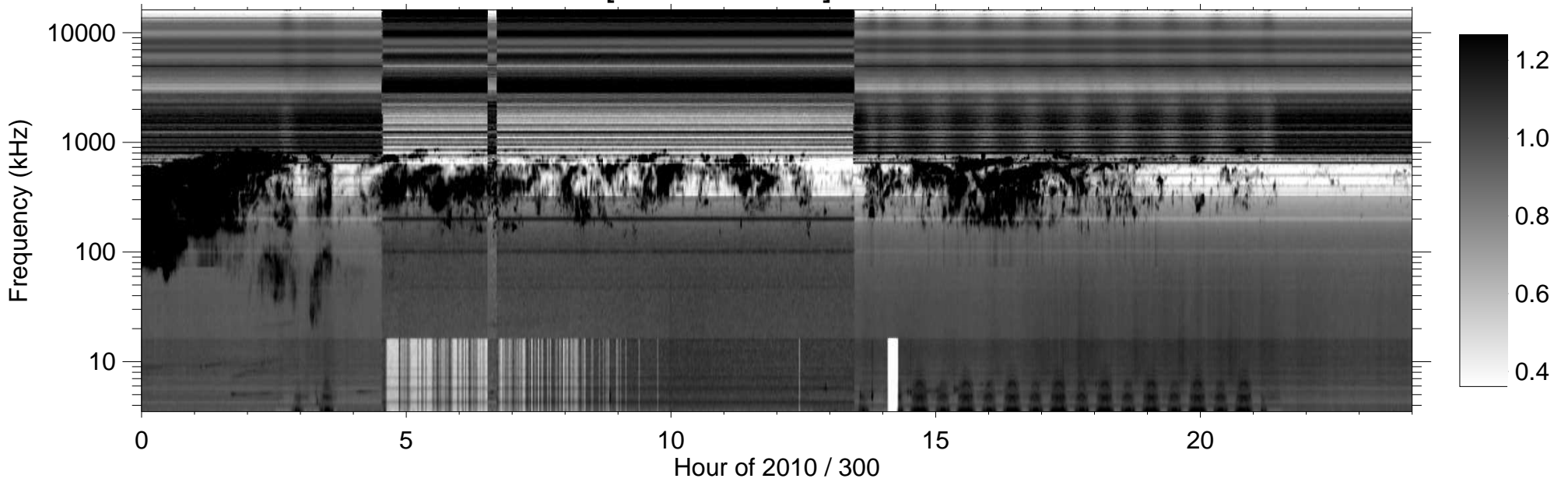
RPWS [ABCH1H2/Ex] (-B) 2010/10/27
