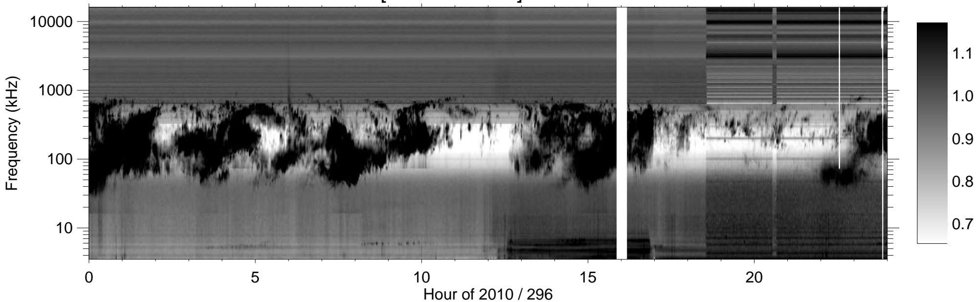
RPWS [ABCH1H2/Ex] (-B) 2010/10/23
