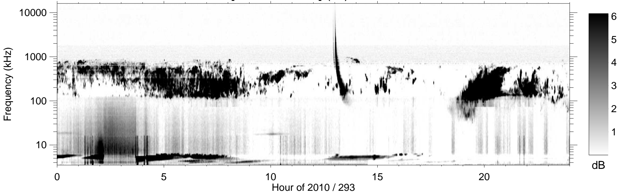
RPWS [ABCH1H2/Ex] (-B) 2010/10/20
