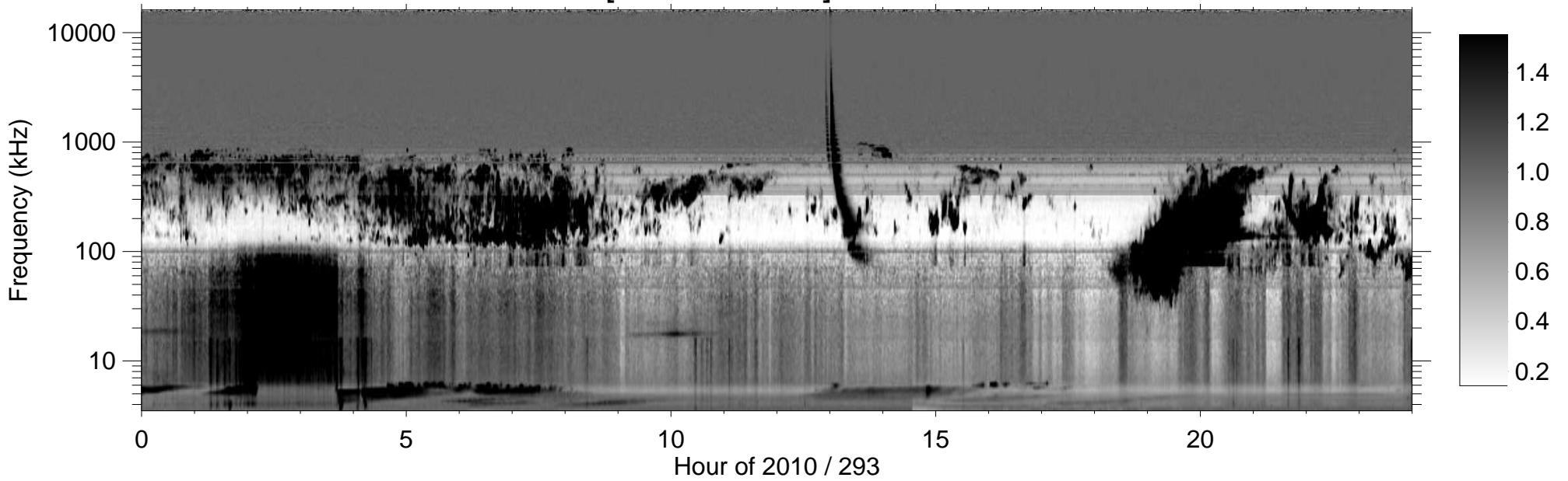
RPWS [ABCH1H2/Ex] (-B) 2010/10/20
