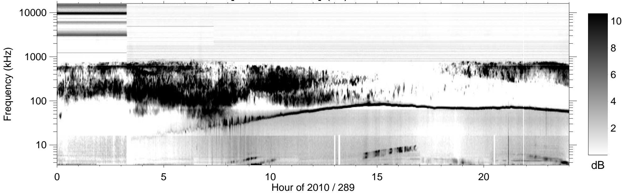
RPWS [ABCH1H2/Ex] (-B) 2010/10/16
