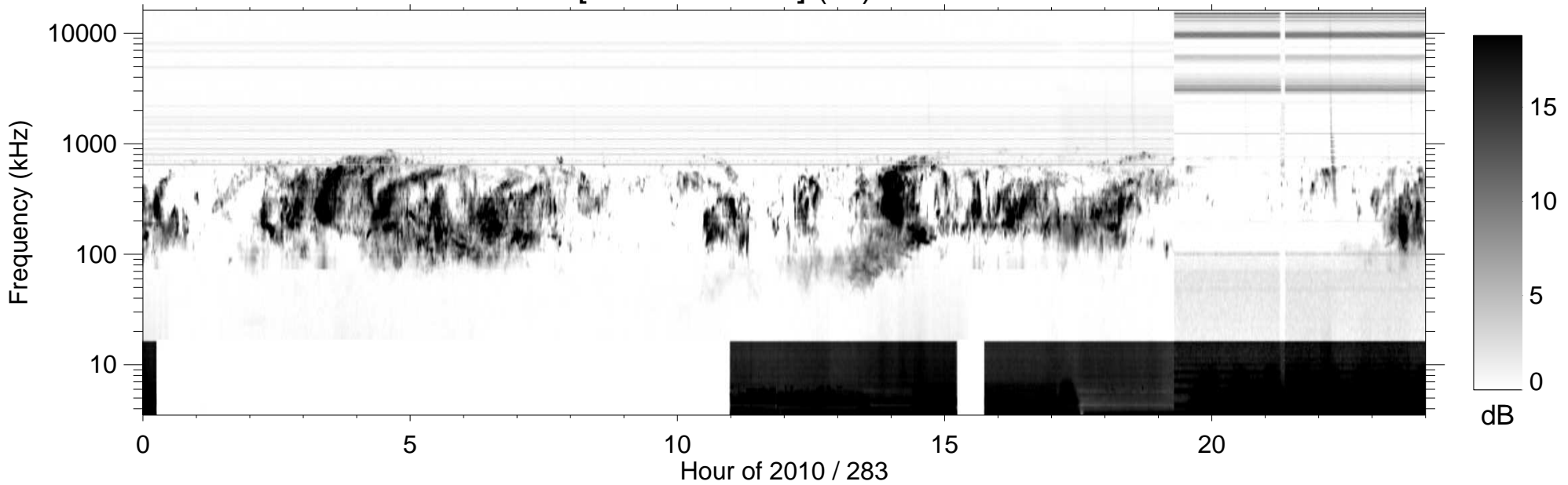
RPWS [ABCH1H2/Ex] (-B) 2010/10/10
