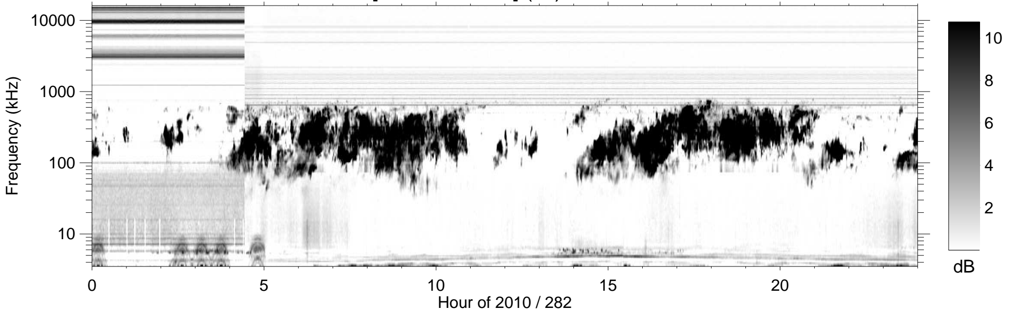
RPWS [ABCH1H2/Ex] (-B) 2010/10/09
