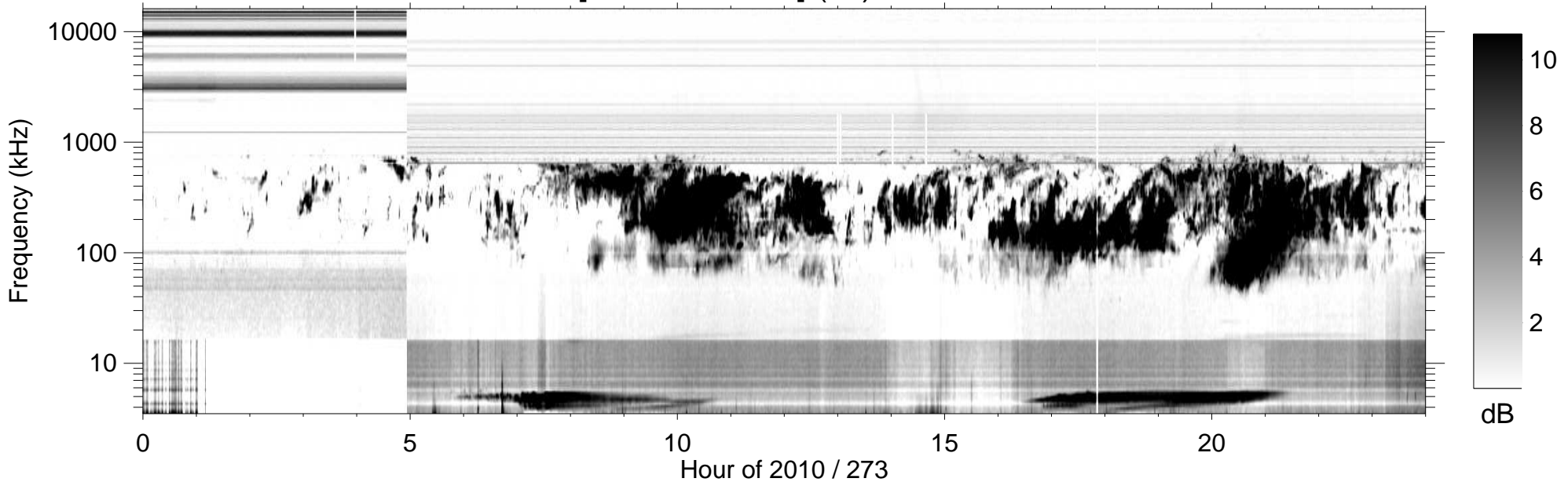
RPWS [ABCH1H2/Ex] (-B) 2010/09/30
