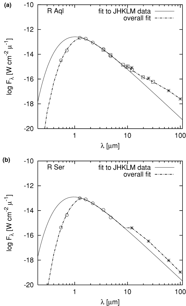
Fig. A.1. Spectral energy distributions of R Aql and R Ser. Circles refer to AAVSO data and present photometry (see Table A.1), squares to the photometry of Epchtein et al. (1980), and asterisks to IRAS (1985) data. The solid line represents the black-body fit to the JHKLM data, and the thick dashed line refers to the overall fit.
